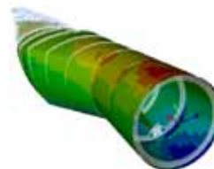
Composite failure analysis of turbine blade
